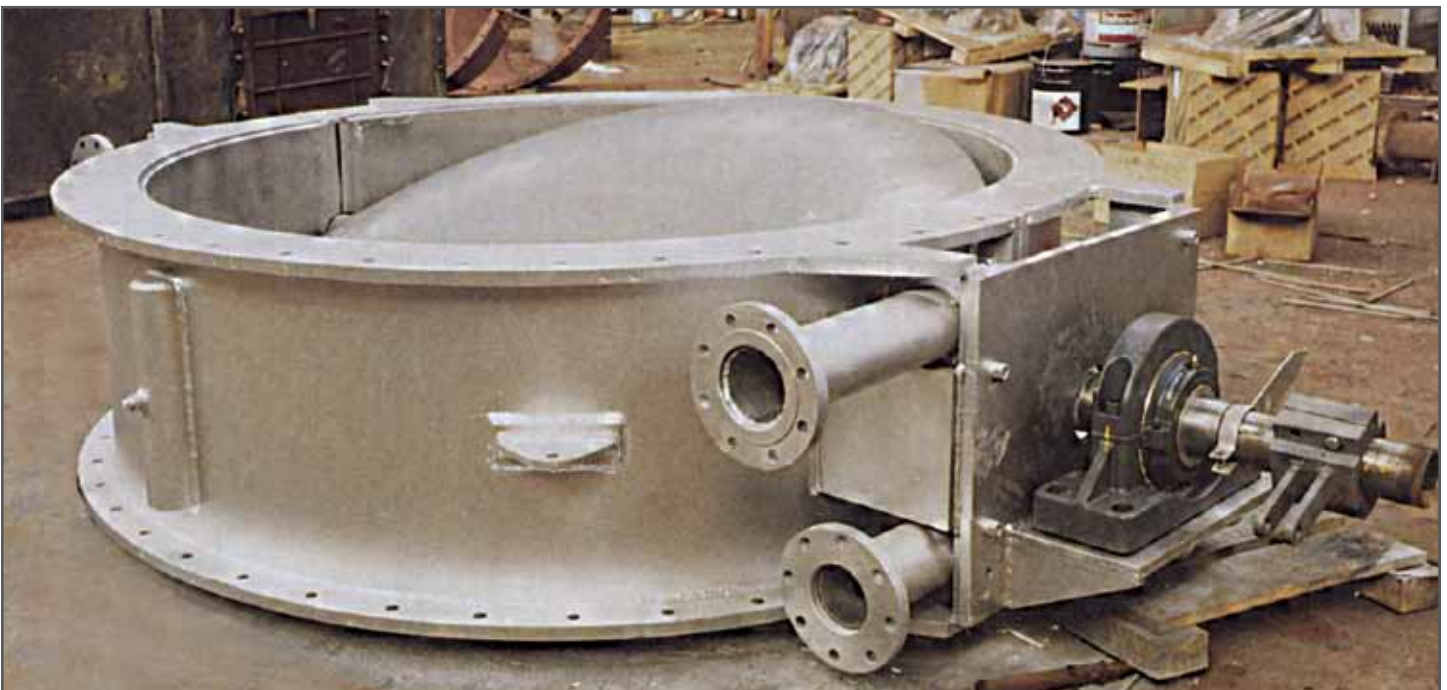
WATER-COOLED BUTTERFLY
